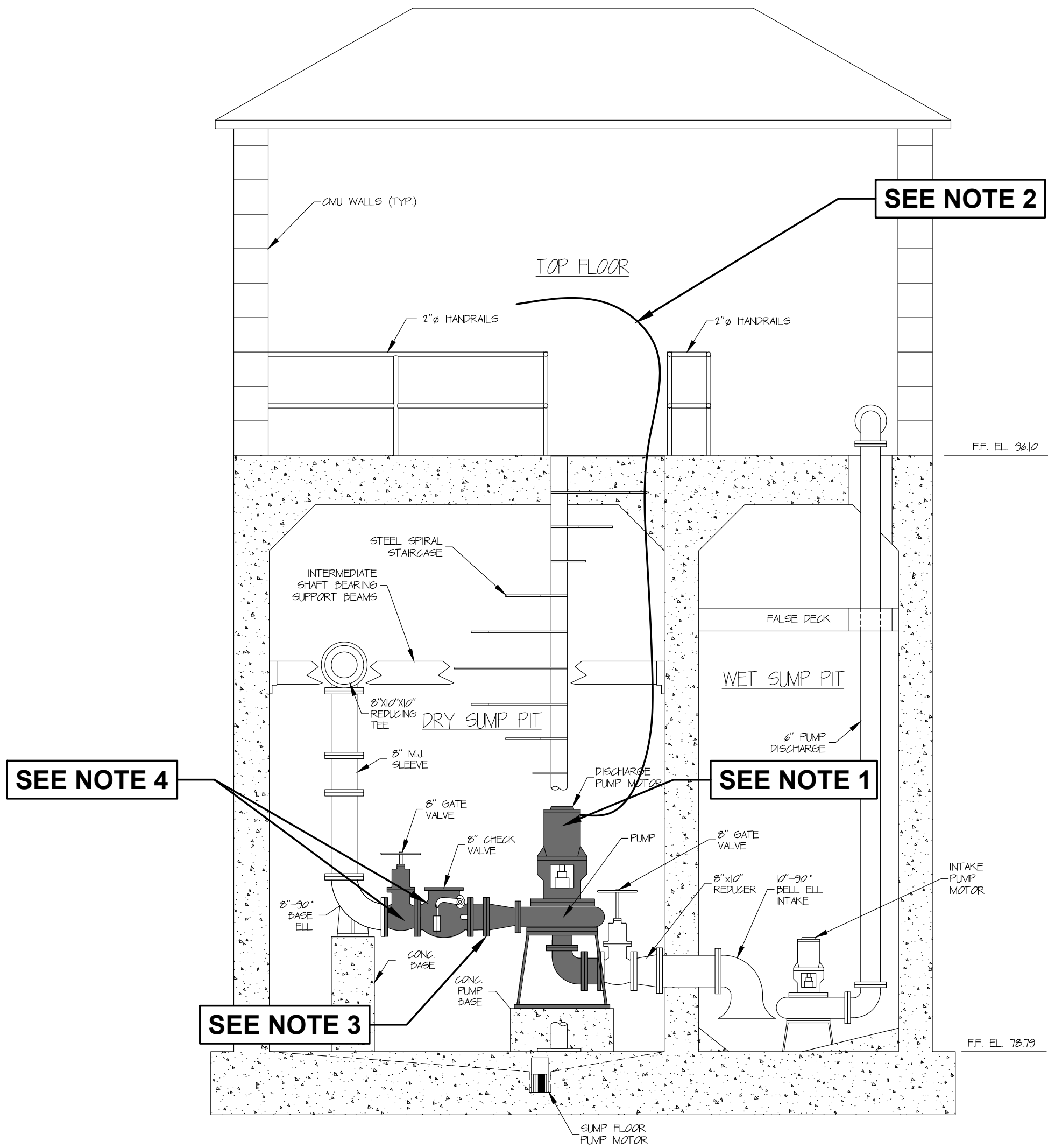
PUMP STATION ELEVATION - SIDE
