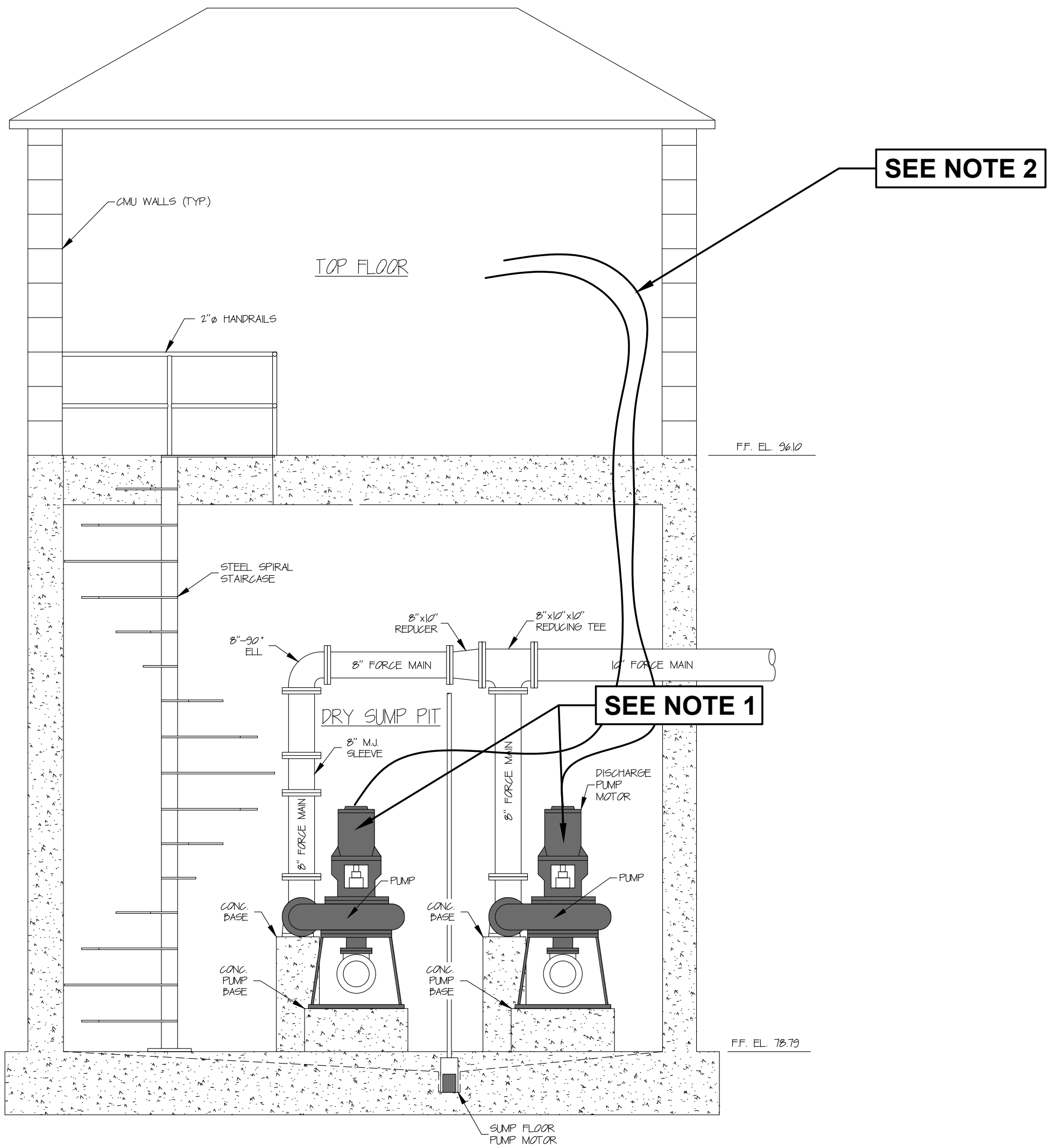
PUMP STATION ELEVATION - FRONT
