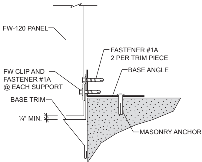
BASE DETAIL WITHOUT SHEETING NOTCH
